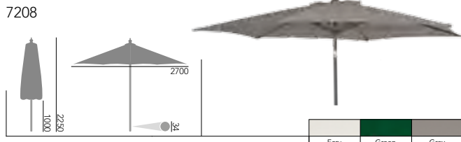
Round Parasol w/ Tilt & Crank 2.7mØ
