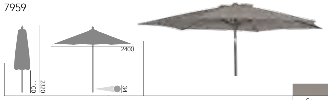
Round Parasol w/ Tilt & Crank 2.4mØ
